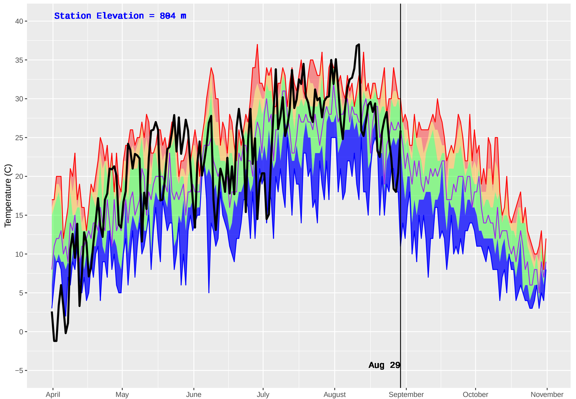
KOOCANUSA (1075) : Historical (2010–2016) and Current (2018) Daily Temperature
